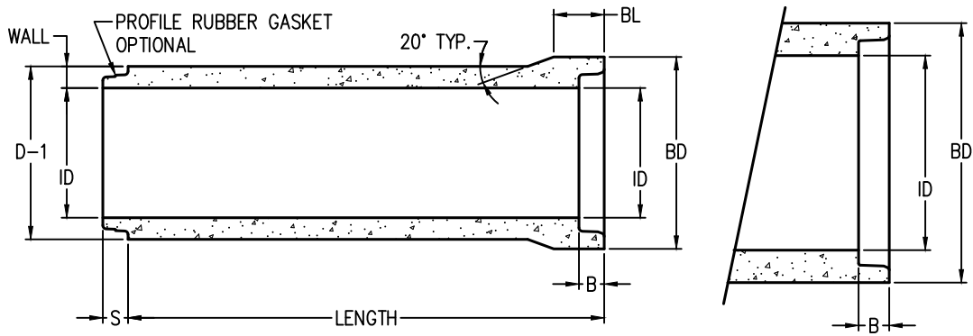
BELL END 42" to 60" PIPE
