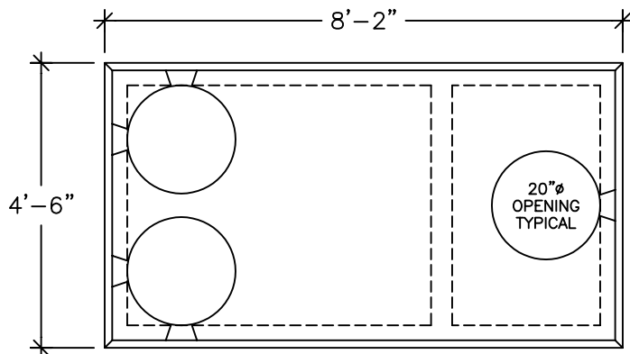
TOP VIEW (COVERS AND RISERS REMOVED)
