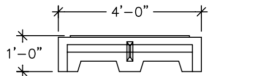
END VIEW (CENTER SECTION) (WALL THICKNESS IS 3") (ROOF THICKNESS IS 3", 5" @ BEAMS)
