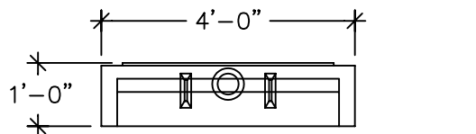
END VIEW (END SECTION) (WALL THICKNESS IS 3") (ROOF THICKNESS IS 3", 5" @ BEAMS)
