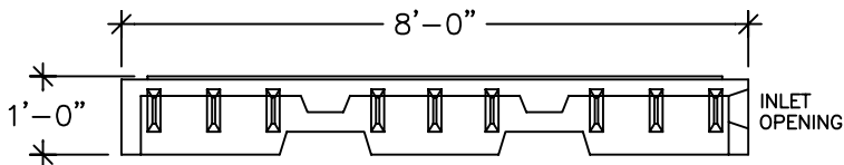
SIDE VIEW (WALL THICKNESS IS 3") (ROOF THICKNESS IS 3", 5" @ BEAMS)
