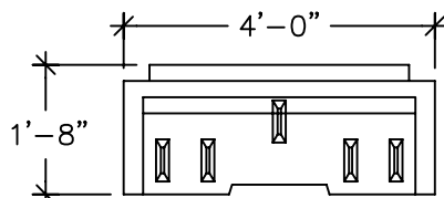
END VIEW (CENTER SECTION) (WALL THICKNESS IS 3") (ROOF THICKNESS IS 5 1/2", 7 1/2" @ BEAMS)
