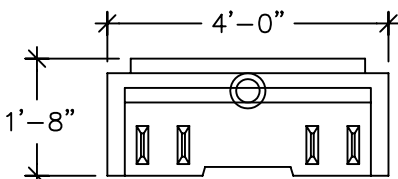
END VIEW (END SECTION) (WALL THICKNESS IS 3") (ROOF THICKNESS IS 5 1/2", 7 1/2" @ BEAMS)
