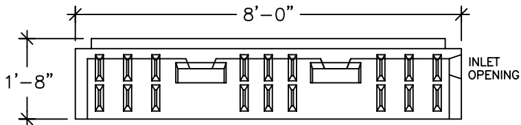
SIDE VIEW (WALL THICKNESS IS 3") (ROOF THICKNESS IS 5 1/2", 7 1/2" @ BEAMS)
