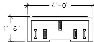
END VIEW (CENTER SECTION) (WALL THICKNESS IS 3") (ROOF THICKNESS IS 3", 5" @ BEAMS)
