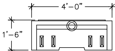
END VIEW (END SECTION) (WALL THICKNESS IS 3") (ROOF THICKNESS IS 3", 5" @ BEAMS)
