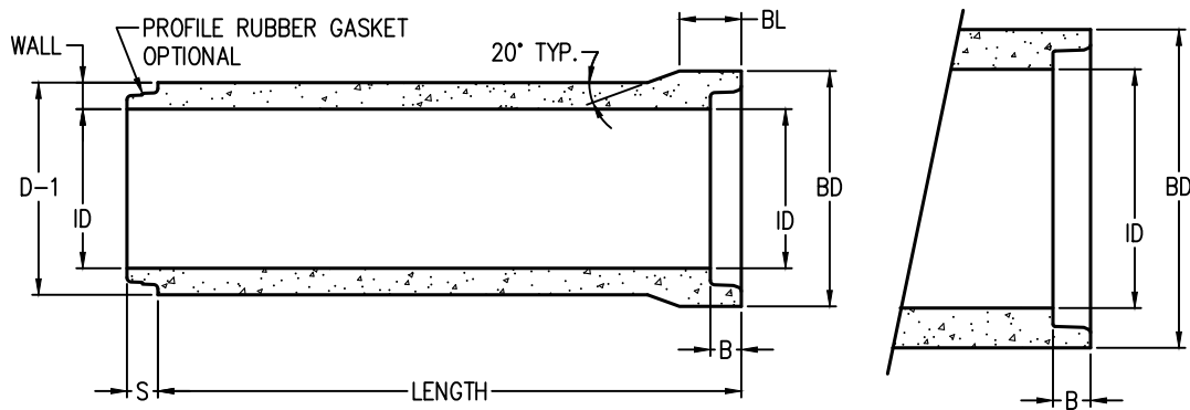
BELL END 42" to 96" PIPE
