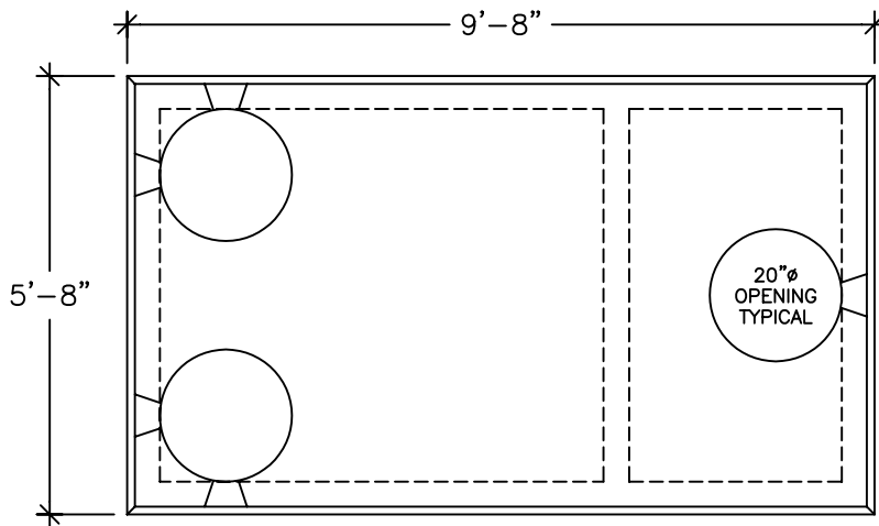
TOP VIEW (COVERS AND RISERS REMOVED)
