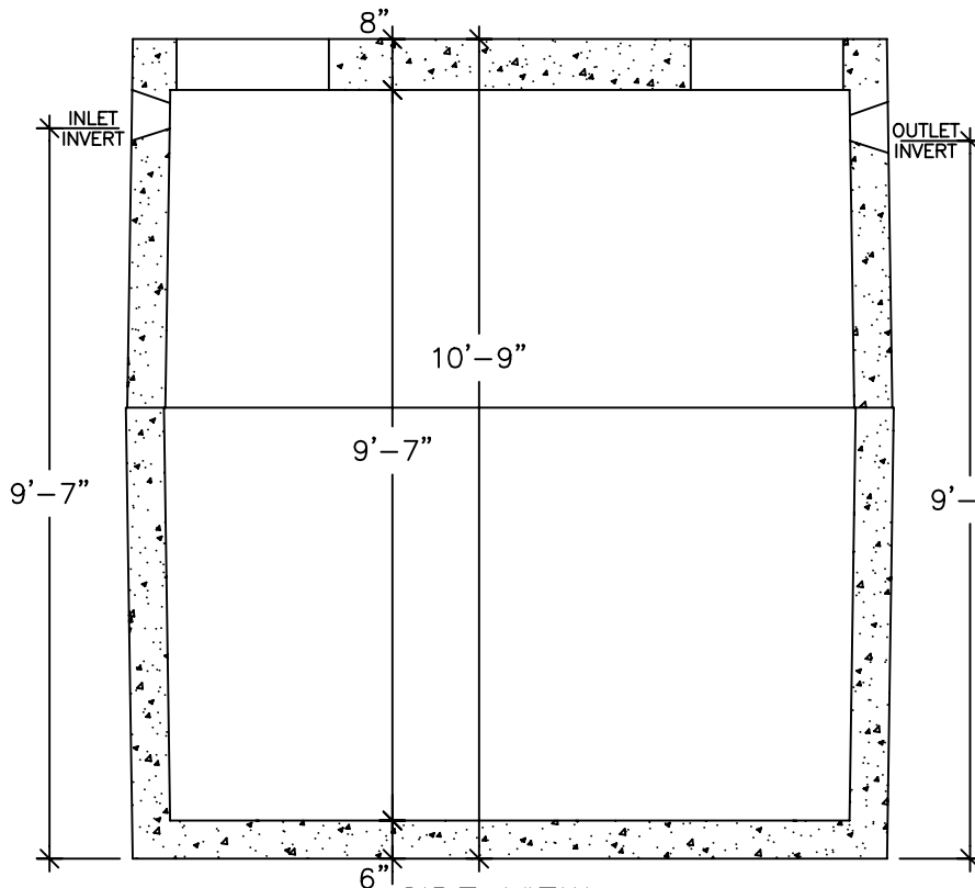
SIDE VIEW
