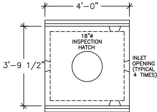
TOP VIEW (ROOF SLAB THICKNESS IS 5")
