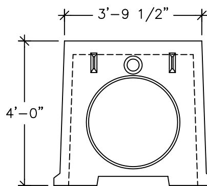
END VIEW (CENTER SECTION) (WALL THICKNESS IS 3")
