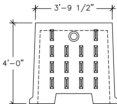
END VIEW (END SECTION) (WALL THICKNESS IS 3")
