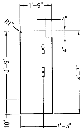
END VIEW
