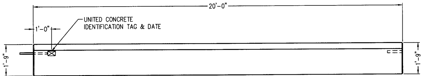
PLAN VIEW
