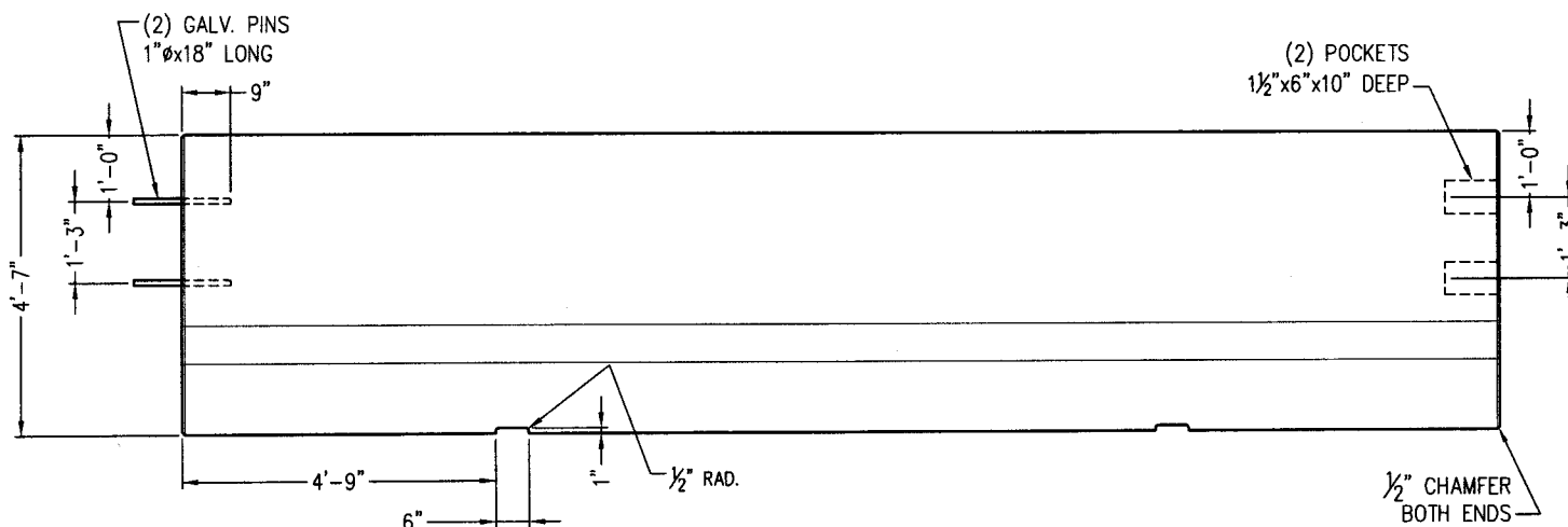
SIDE VIEW
