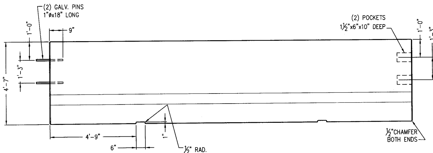
SIDE VIEW
