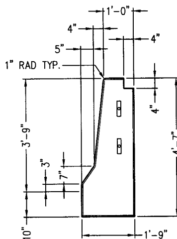
END VIEW
