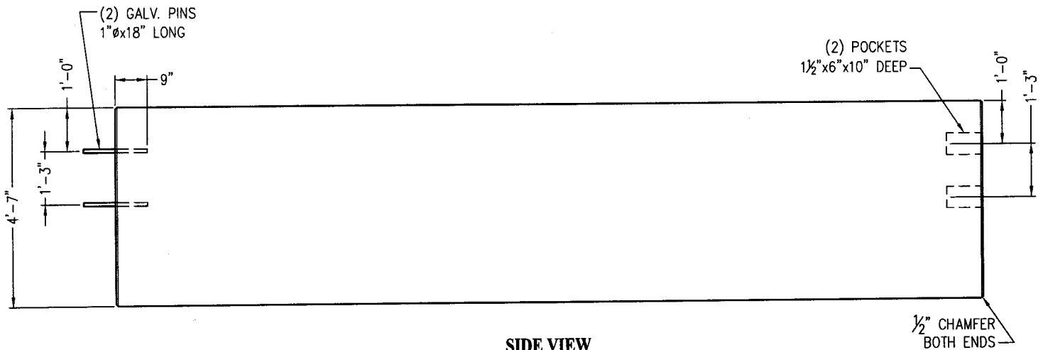
SIDE VIEW
