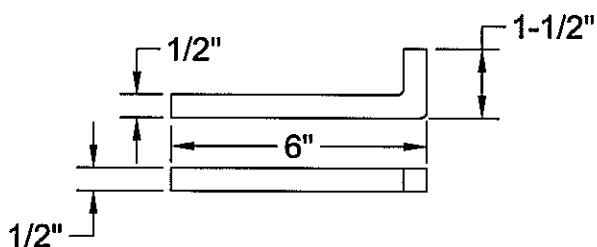
STAINLESS STEEL HOOK (2 EACH REQUIRED PER HOOD)
