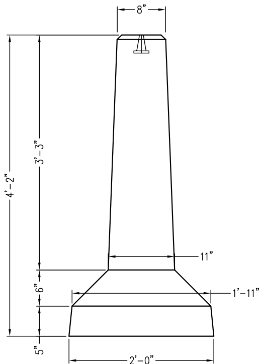
ELEV. VIEW
