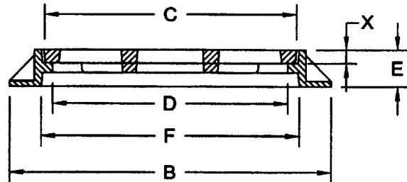
FRAME SHOWN WITH TYPE 'C' GRATE
