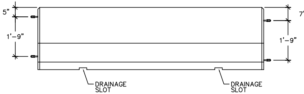
SIDE ELEVATION
