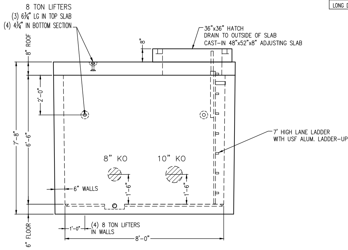
SIDE VIEW
