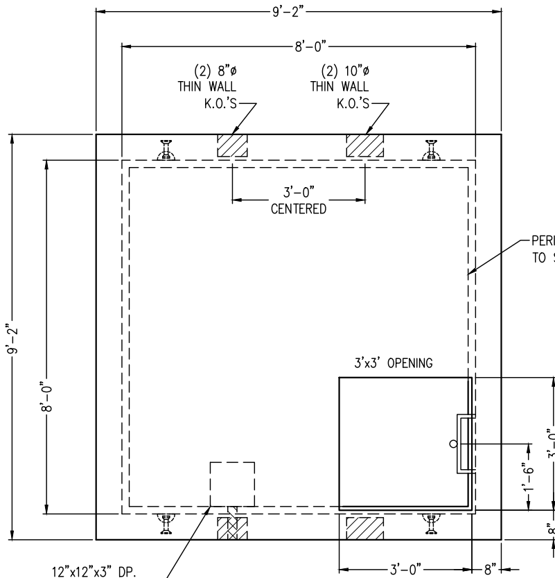
TOP VIEW
