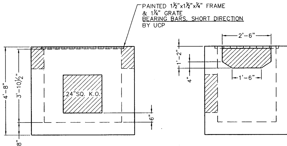
WALL A
