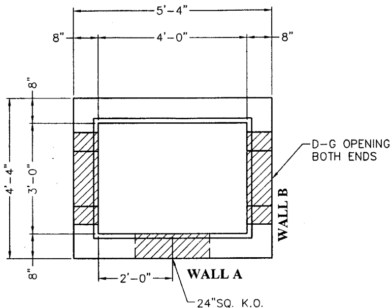
PLAN VIEW (SHOWN W/O GRATE)
