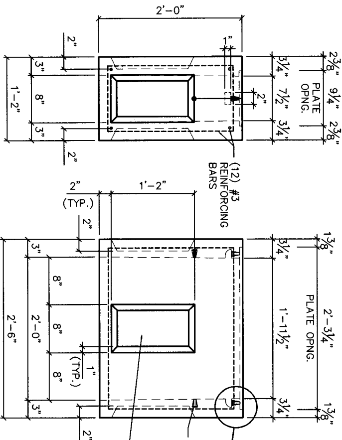
ELEVATION "A"
